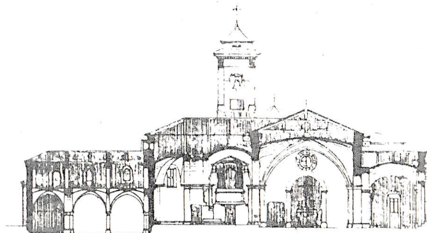
Fianco — Scala 1 a 200
