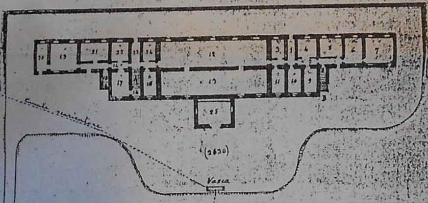
Piano terreno
