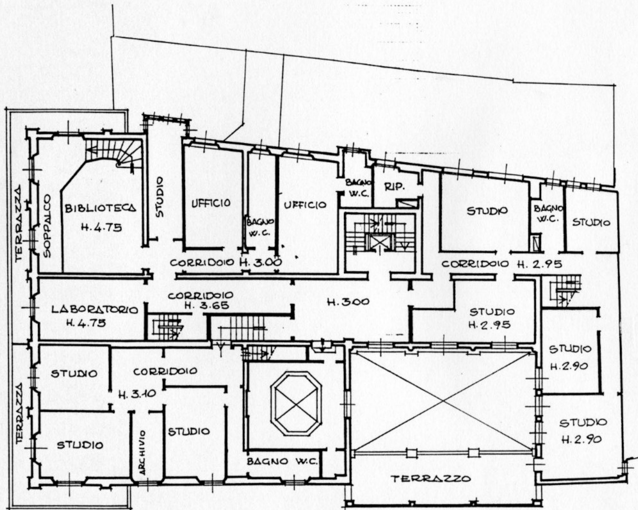
PIANO QUARTO
