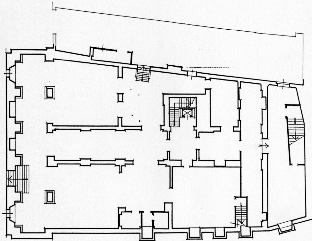
PIANO SEMINTERRATO
